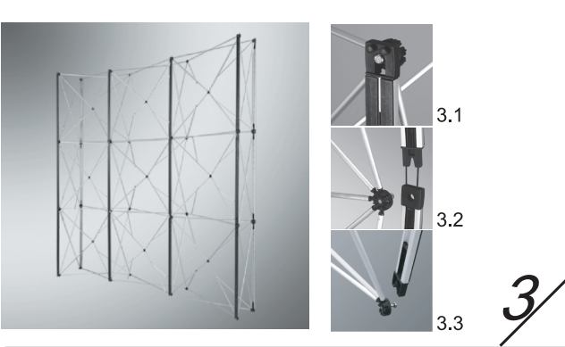
3,Draw the magnetic poles separately to make its hole fit with the tip on the frame one by one.Attention:keep the circlip for hole from bottom to top with the frame while assembling.
